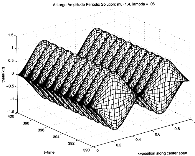
Fig. 5 Long term response to the initial conditions (13)
