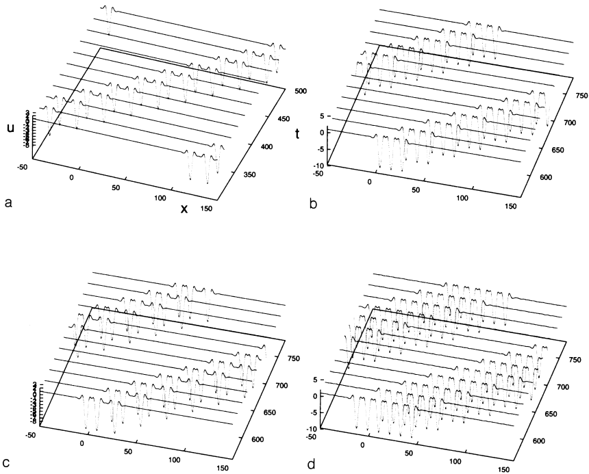
Fig. 10 Simple and complicated stable solutions; numerical solutions to (14) with nonlinearity (17) using the fixed grid method with initial conditions for c = 1.1 which are exact solitary waves that appear to be stable: (a) the 2(5) ; (b) the 3(3, 3) ; (c) the 3(3, 5) (note this is an asymmetric wave); and (d) the 6(3, 3, 3, 3, 3) . In each case the solution is plotted after a time interval which is sufficient for any transient instabilities to develop
