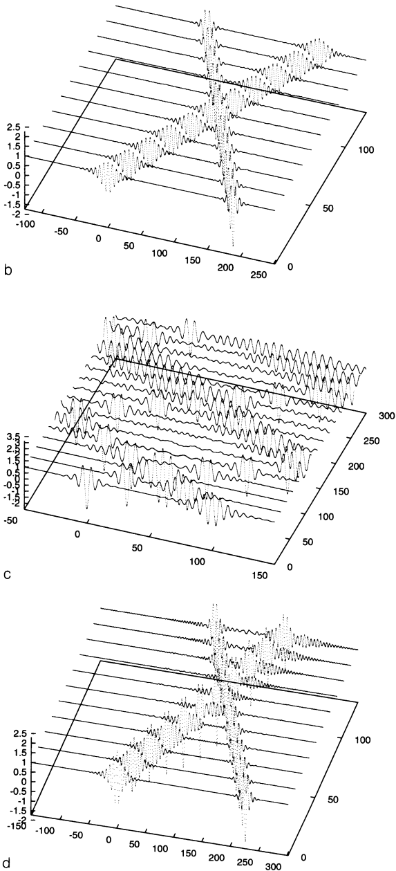
Fig. 13 Passage of primary solitary wave solutions to (14) with |c|=1.354 and 1.4 through each other. (a), (b) With the exponential nonlinearity (17), using respectively the fixed and moving grid methods. (c), (d) With the piecewise linear term (15) using respectively the fixed and moving grid methods. Moving grid computations were performed using 2001 grid point
