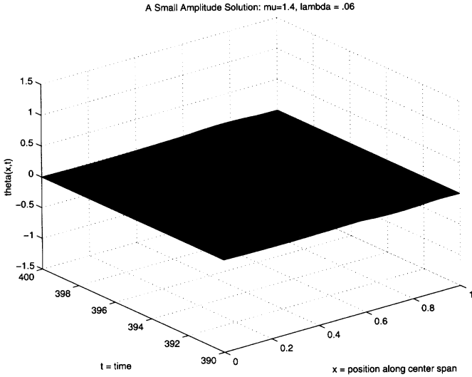
Fig. 4 Long term response to the initial conditions (12)
