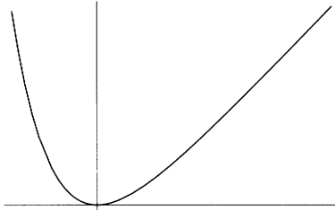
Fig. 1 Toda potential V(r)
